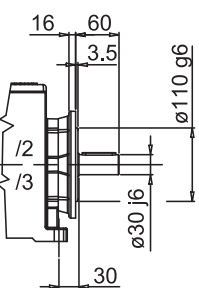
Modular Flange Bride modular
