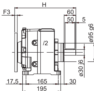
Modular Flange Bride modular
