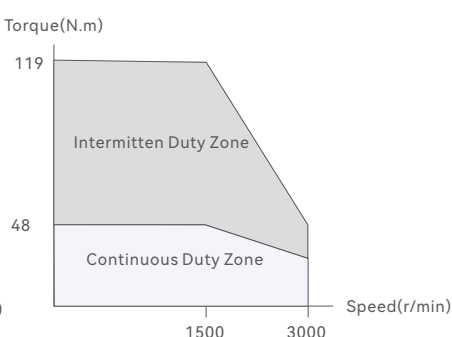
7500W Motor
