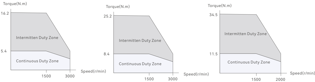
850W Motor
