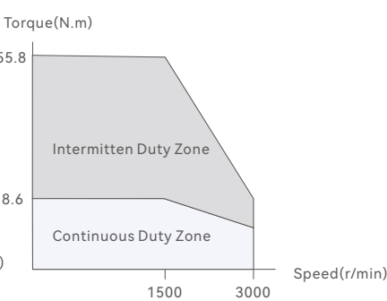
2900W Motor
