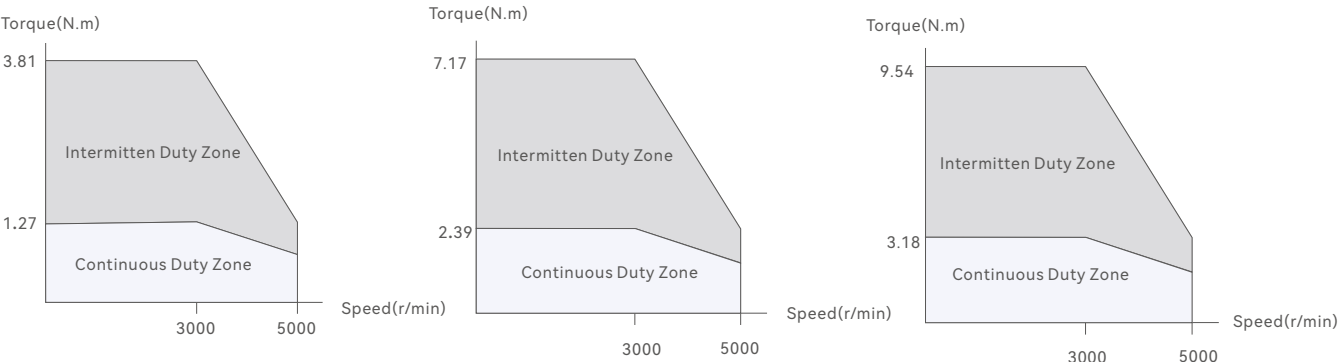
400W Motor
