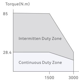
4400W Motor
