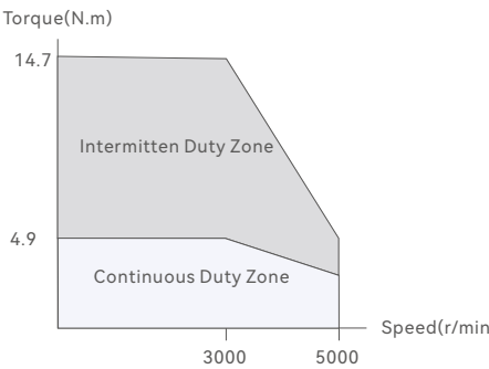
1500W Motor
