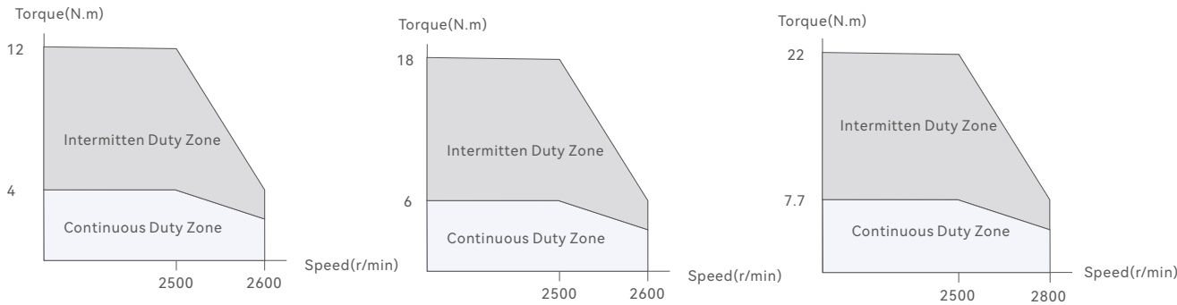
1000W Motor
