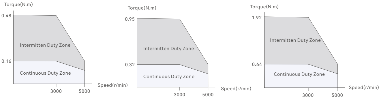
50W Motor
