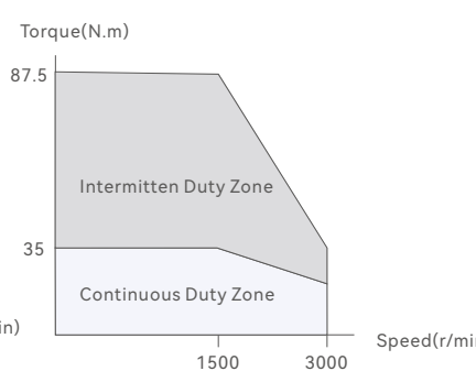
5500W Motor
