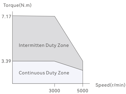
750W Motor
