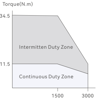
1800W Motor
