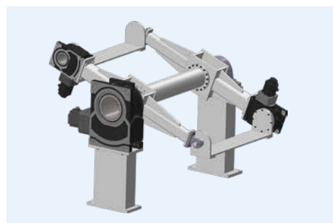
Ferris-wheel type welding positioner
