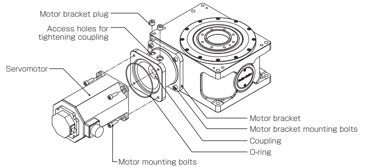
Servomotor installation schematic(Standard gear ratio model)
