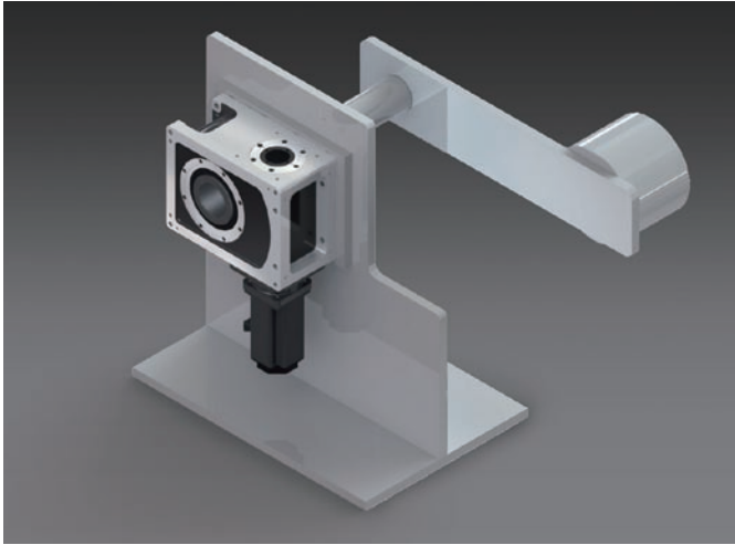
Oscillating Work with Off-Center Loads
