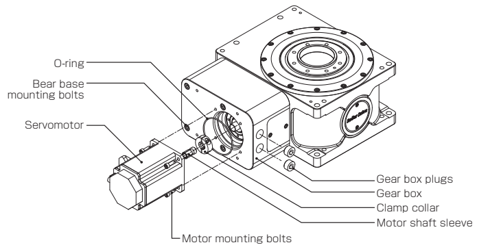
Servomotor installation schematic(High gear ratio model)
