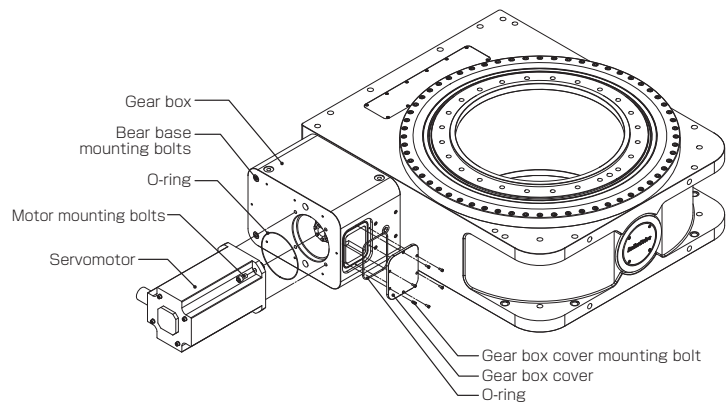
Servomotor installation schematic(High gear ratio model)
