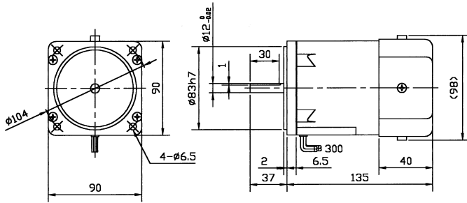
Fig.2 GEARED MOTOR
